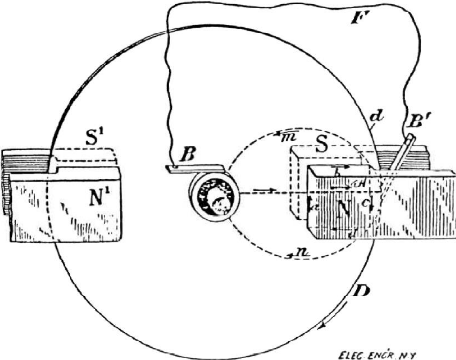
General schematic of a homopolar generator.
