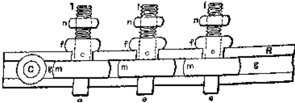
FIG. 6 -- DISCHARGER WITH MULTIPLE GAPS.
