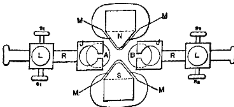
FIG 4 -- ARRANGEMENT OF IMPROVED DISCHARGER AND MAGNET.
