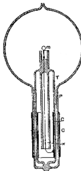
Fig. 22 – TYPE OF BULB WITHOUT LEADING-IN WIRE
