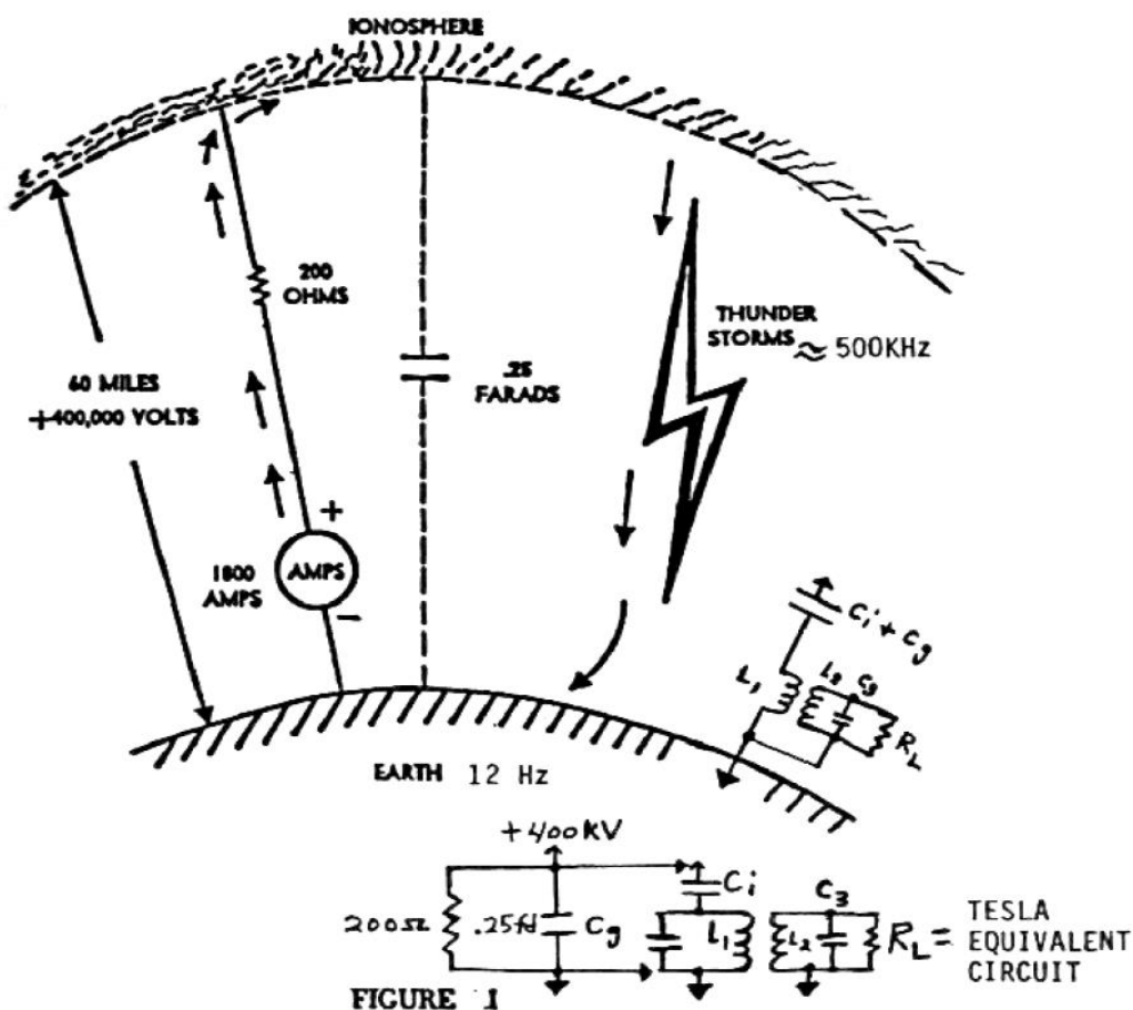
Equivalent circuit of earth's electrostatic voltage field.
