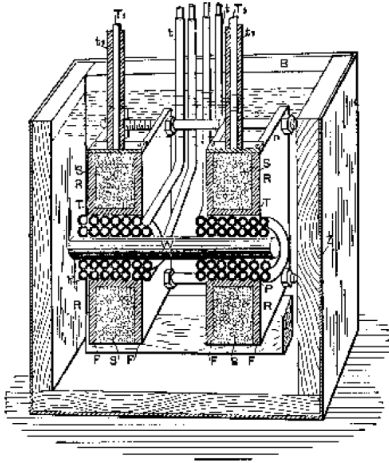
FIG. 3 -- DISRUPTIVE DISCHARGE COIL.
