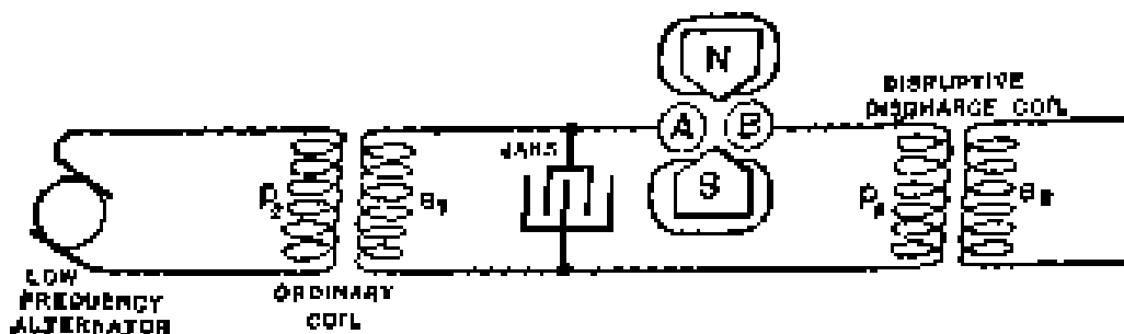
FIG. 5 -- ARRANGEMENT WITH LOW-FREQUENCY ALTERNATOR AND IMPROVED DISCHARGER.
