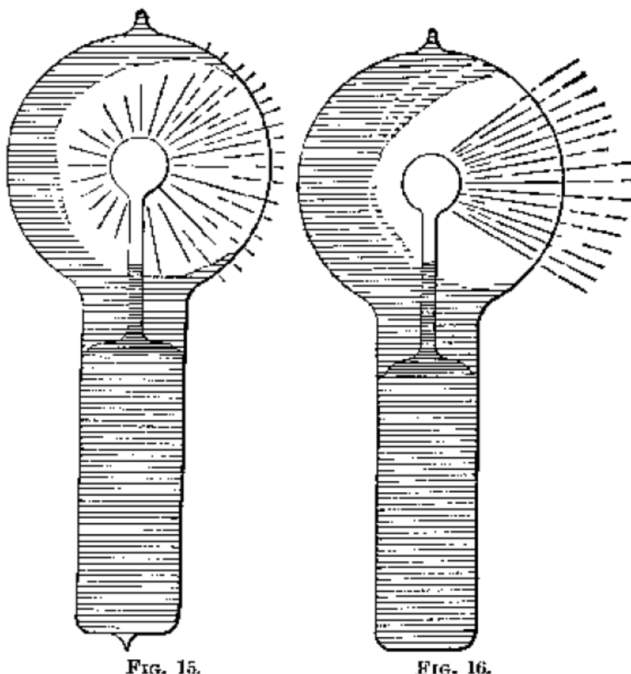
FORMS AND PHASES OF THE ROTATING BRUSH
