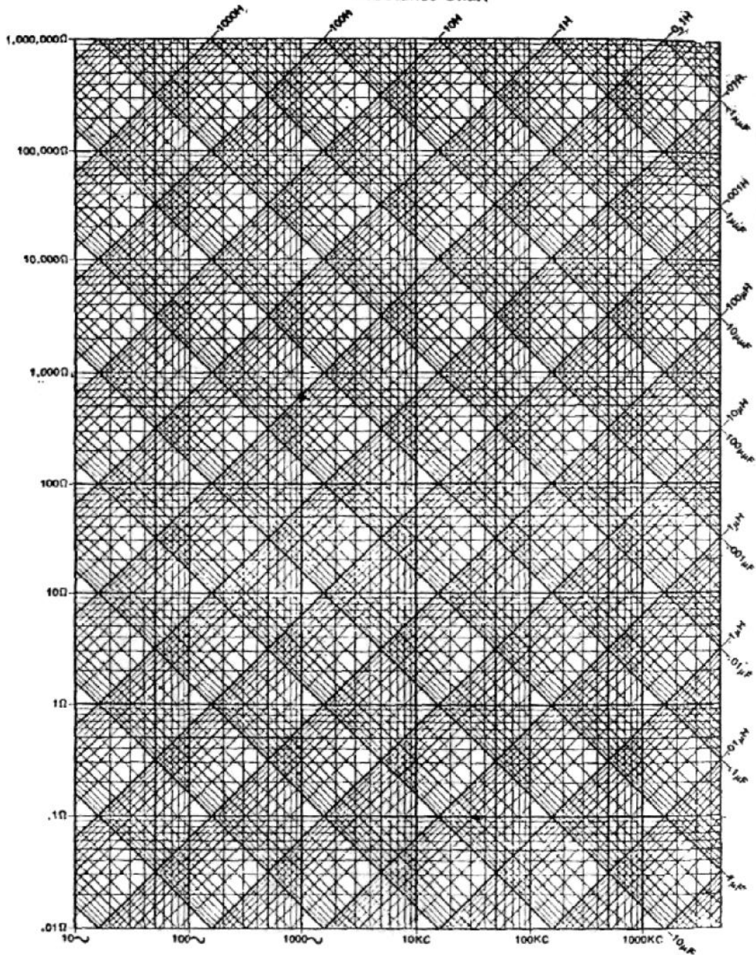
Reactance Chart
