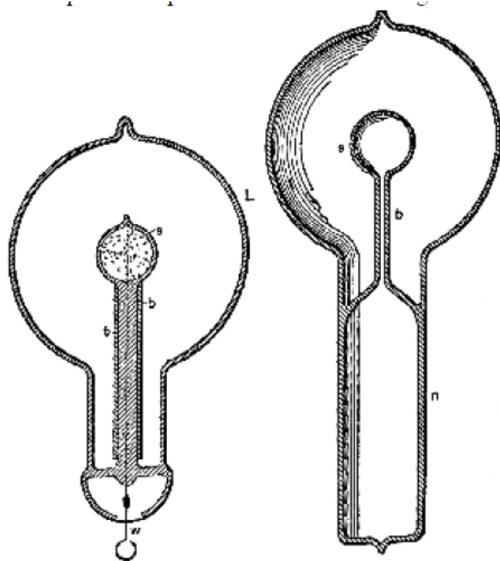
FIG. 12. FIG. 13. BULBS FOR PRODUCING ROTATING BRUSH.
