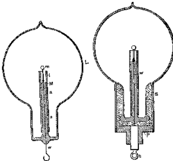
Fig. 18 – BULB WITH MICA TUBE AND ALUMINIUM SCREEN
