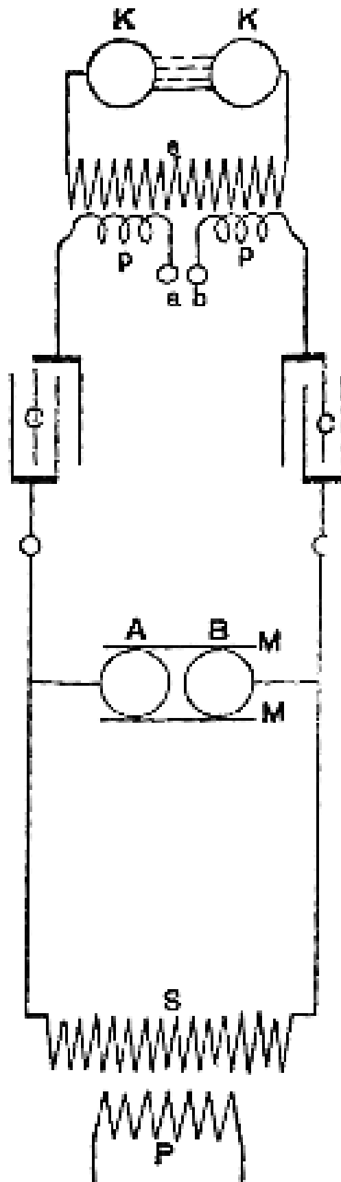
FIG. 2 -- IMITATING THE SPARK OF A-HOLTZ MACHINE.
